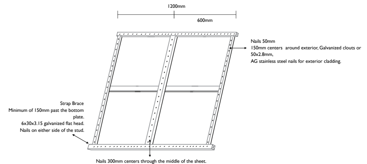
Figure 4: BRACING TEST
