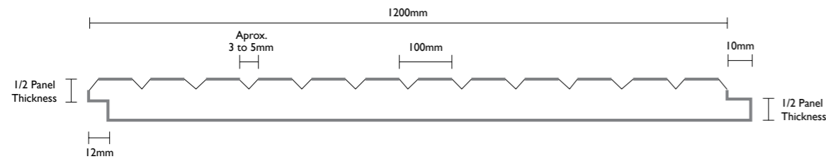
Figure 3: V-GROOVE PROFILE 100mm ON CENTRE
