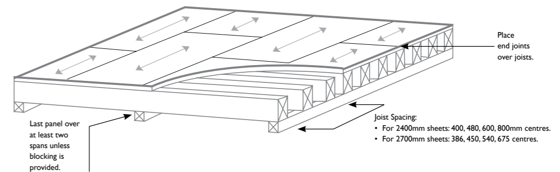
Figure 1: ARAUCO FLOORING LAYOUT
